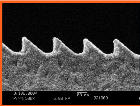
High Blaze Angle Grating, 300nm Pitch
