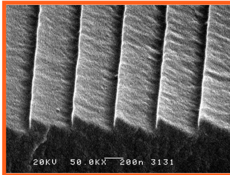
Blazed Grating, 400nm Pitch
