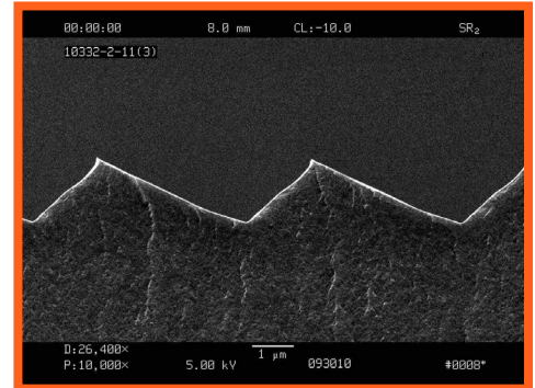
Blazed Grating, 5.2 µm Pitch
