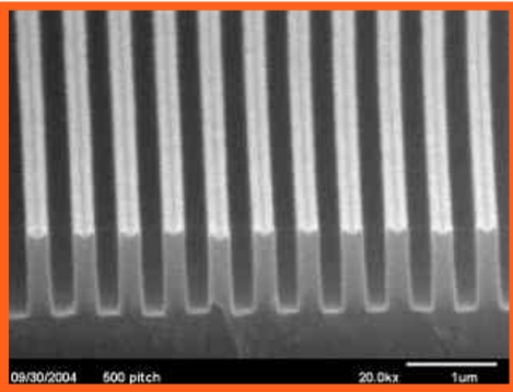
Representative SEM of 2000 l/mm grating profile
